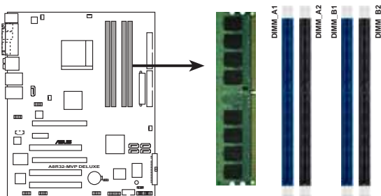
A8R32-MVP DELUXE 184-pin DDR DIMM sockets
