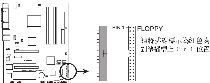
A8R32-MVP DELUXE Floppy disk drive connector
