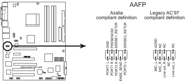
A8R32-MVP DELUXE Analog front panel connector
